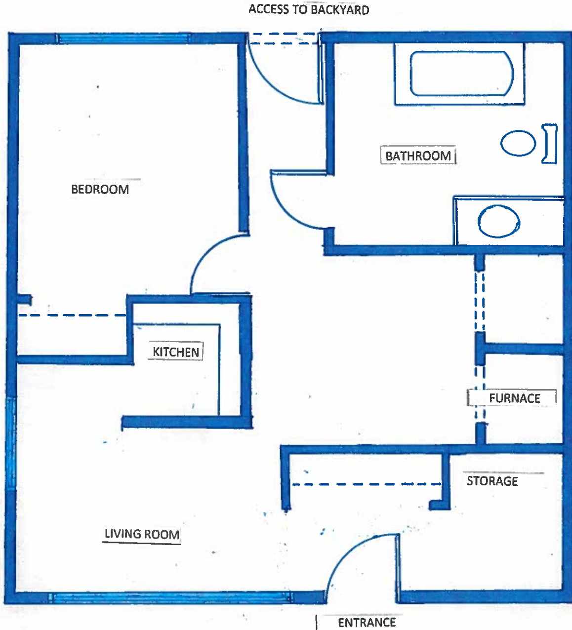
Pioneer Haven Floor Plan
